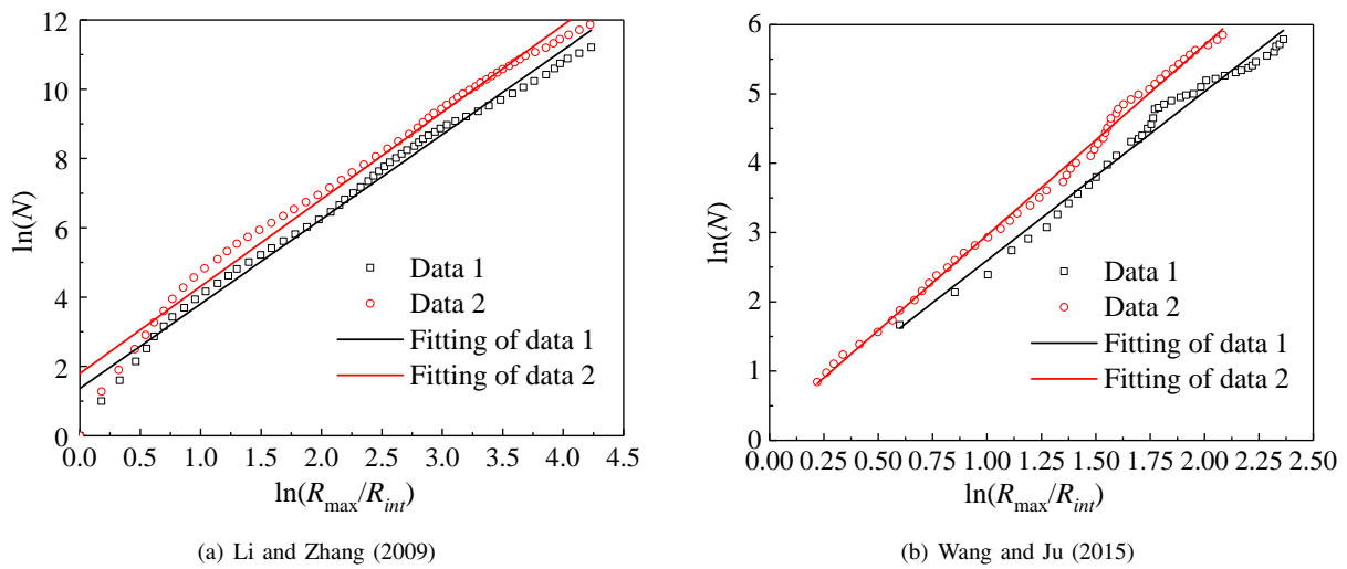
Fig. 2. The fractal pore size distribution.
