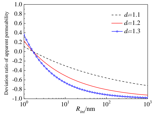
(b) Deviation ratio of apparent permeability
