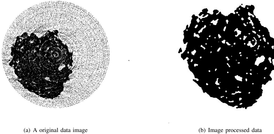
Fig. 1. Image Processing.
