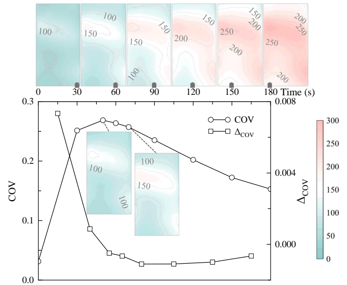
Fig. 4. Variation in surface temperature distribution and COV of granite B under microwave irradiation.
