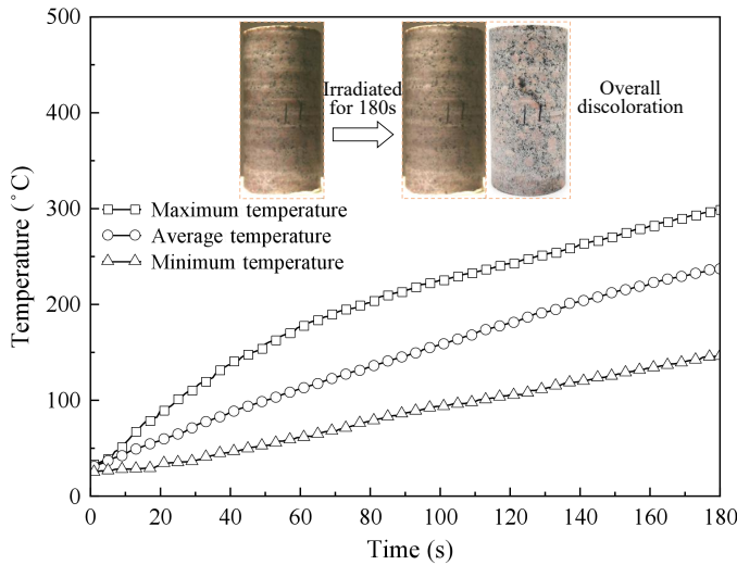
Fig. 3. Temperature curves and fracture characteristics of granite B surface under microwave irradiation.
