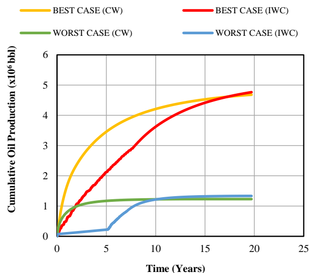
Fig. 13. FOPT comparison of IWC and CW under porosity variations.
